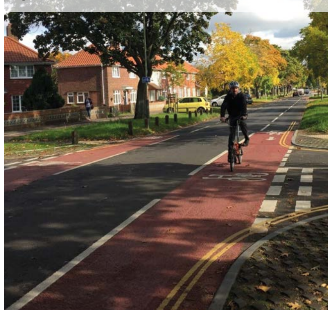
Figure 6.21: Centre line removal, Norwich
